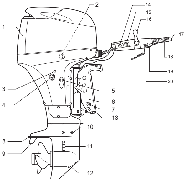
DF40ATH/QH/50ATH/60ATH
